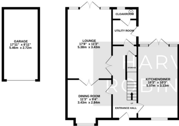
GROUND FLOOR 839 sq.ft. (77.9 sq.m.) approx.
